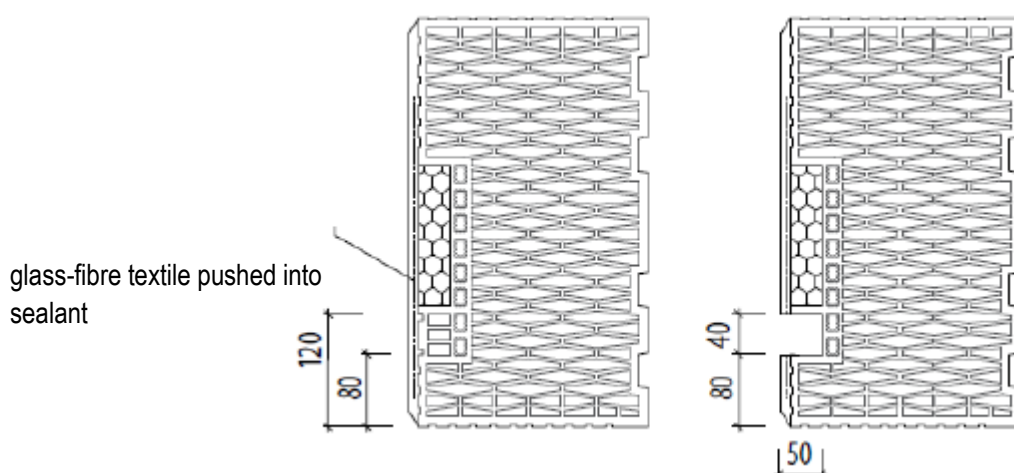
Setting up jamb
