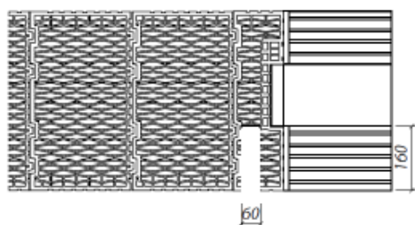
Making a pocket of rear PVC cover
